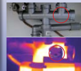
The blockage in this pipe is quickly located using a thermal camera. Action will be taken before the problem worsens.
